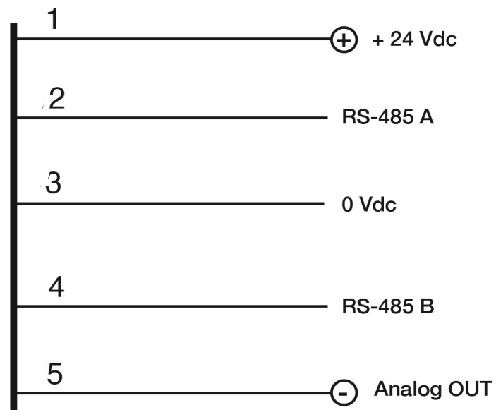
Connector
