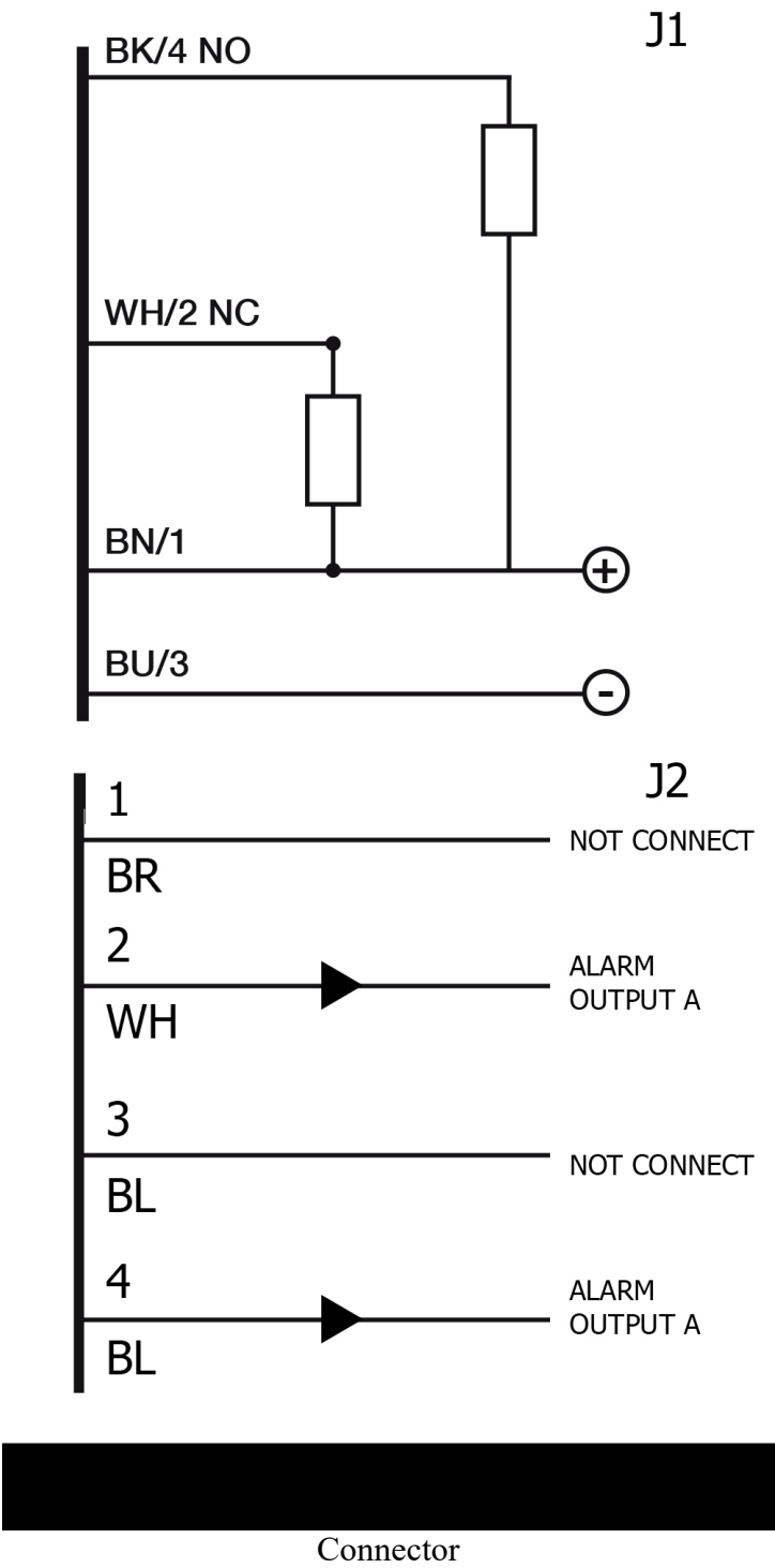
Eletrical diagram
