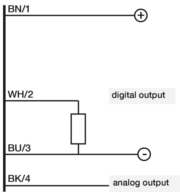
Eletrical diagram
