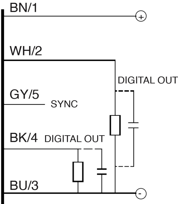
Eletrical diagram
