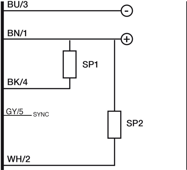
Eletrical diagram
