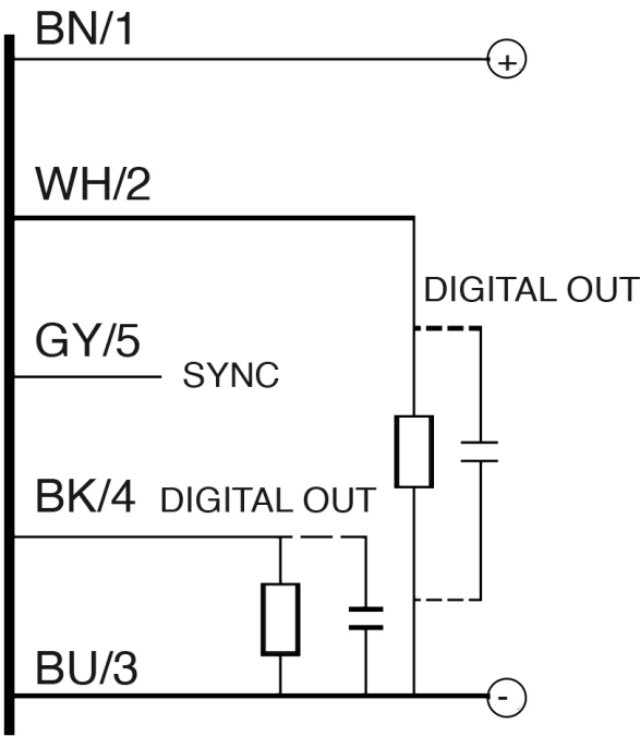
Eletrical diagram
