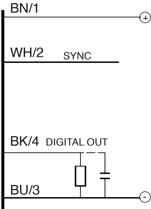
Eletrical diagram
