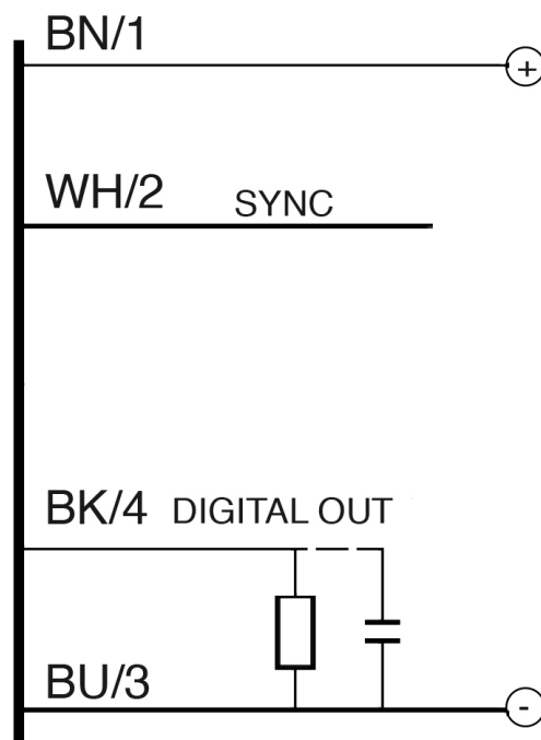
Electrical diagram
