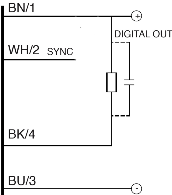
Eletrical diagram
