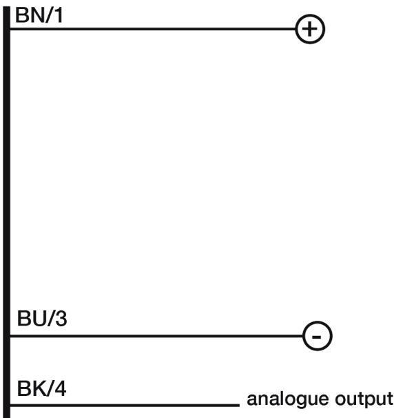
Eletrical diagram
