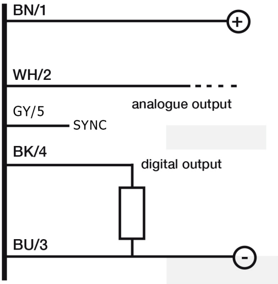
Eletrical diagram
