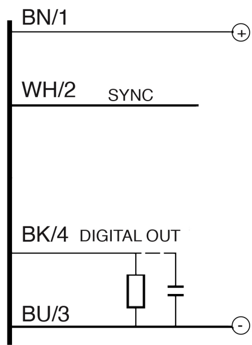
Eletrical diagram
