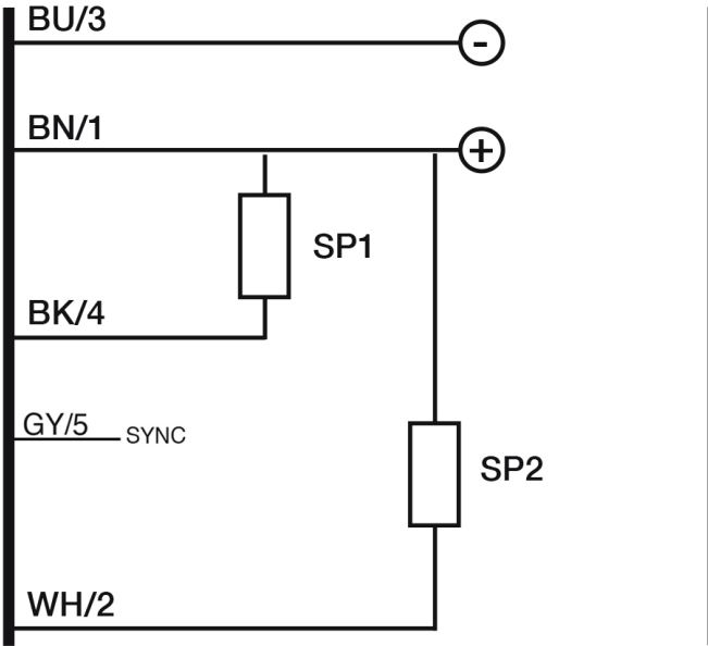
Eletrical diagram
