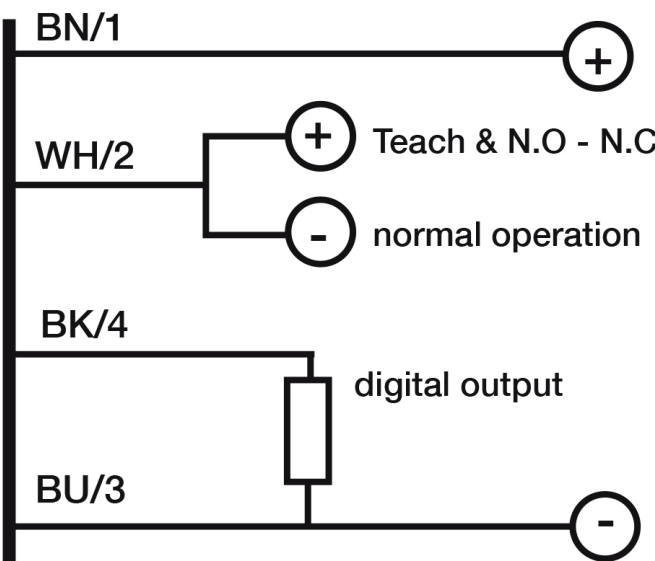
Eletrical diagram
