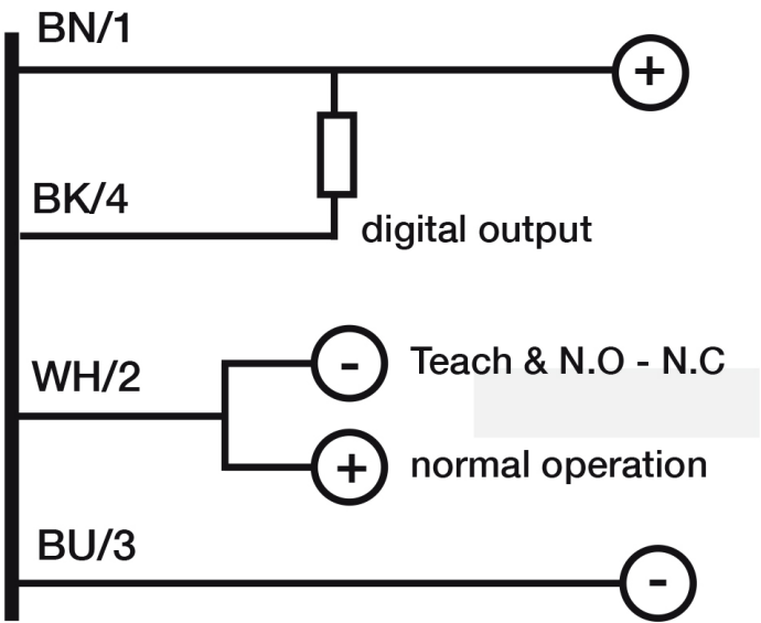
Eletrical diagram
