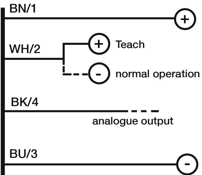
Eletrical diagram
