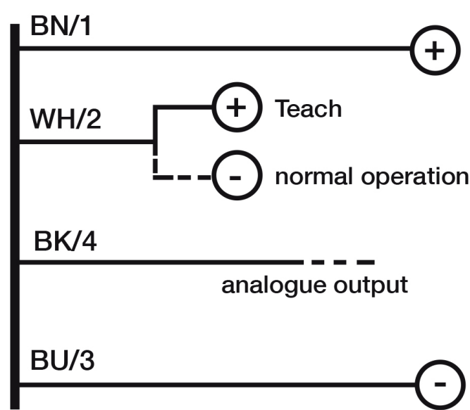
Eletrical diagram
