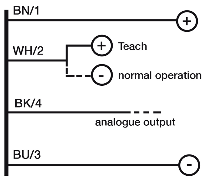
Eletrical diagram
