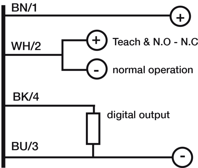
Eletrical diagram
