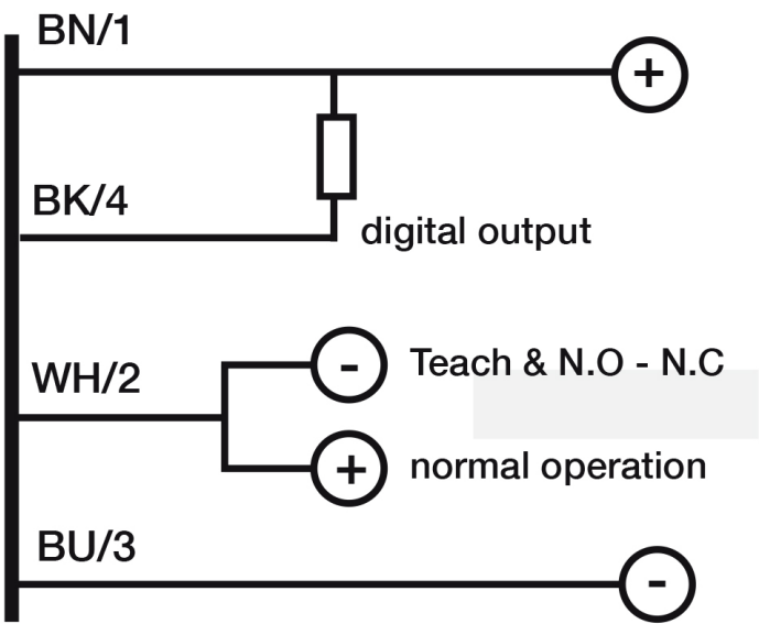
Eletrical diagram
