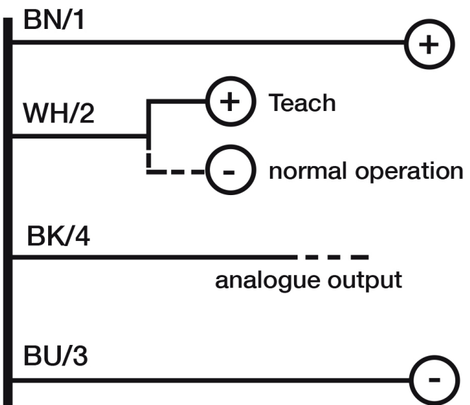
Eletrical diagram
