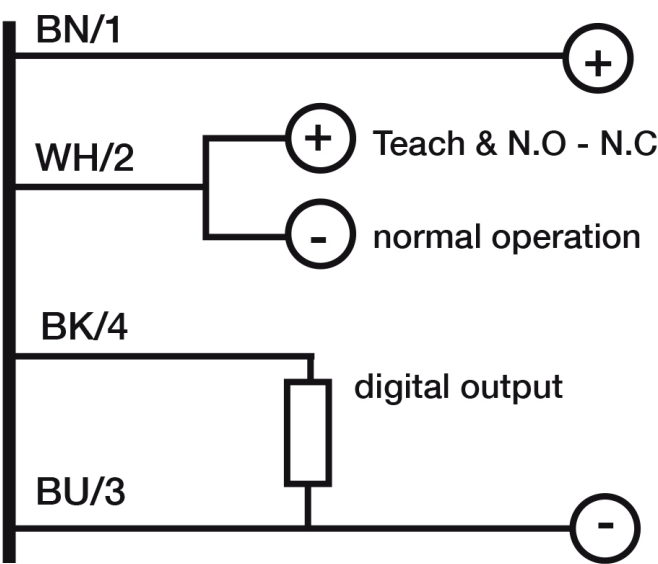
Eletrical diagram
