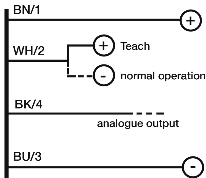
Eletrical diagram
