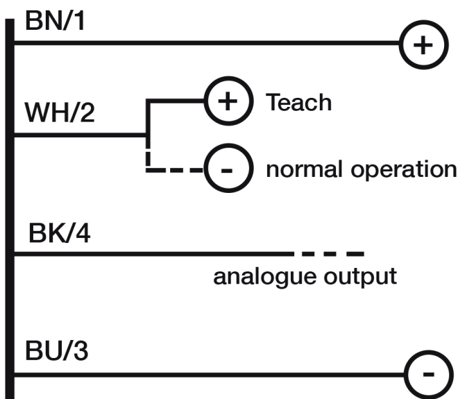
Eletrical diagram
