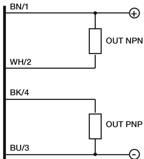
Electrical diagram
