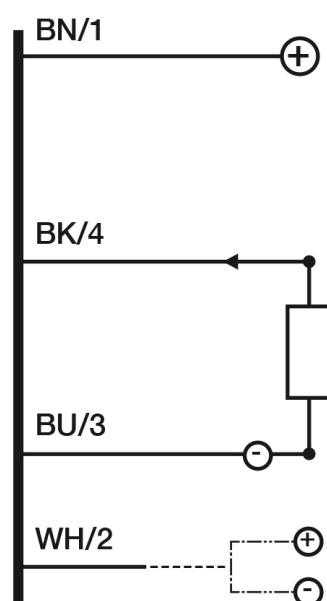
Electrical diagram
