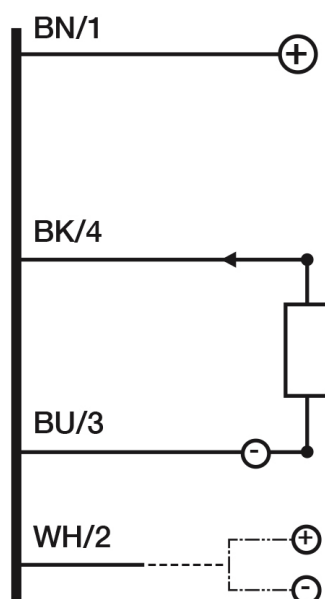
Electrical diagram
