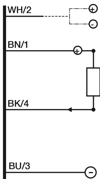
Connector
