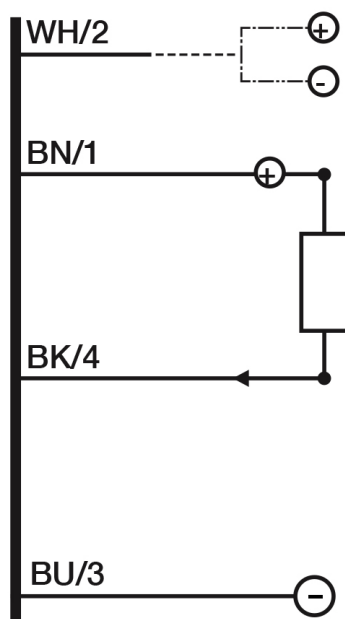
Eletrical diagram
