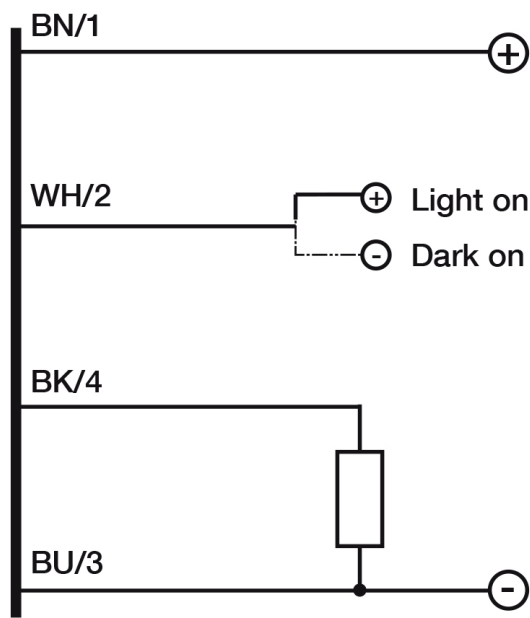
Eletrical diagram
