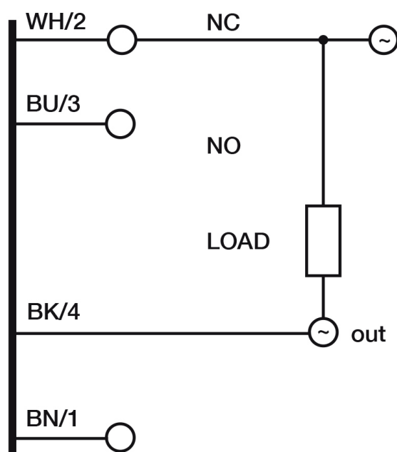
Eletrical diagram
