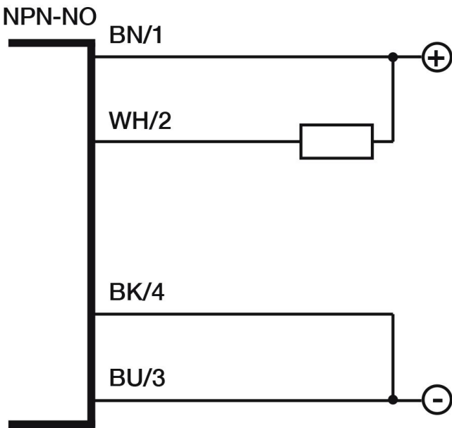
Eletrical diagram
