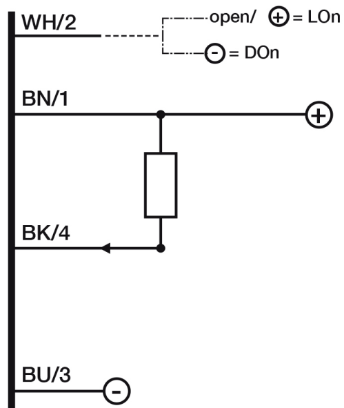
Electrical diagram
