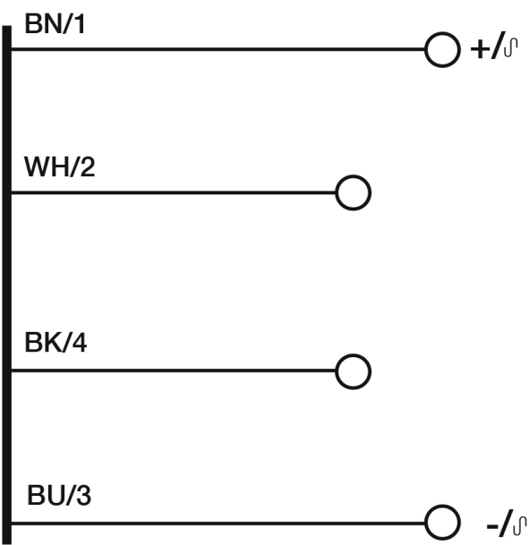
Eletrical diagram
