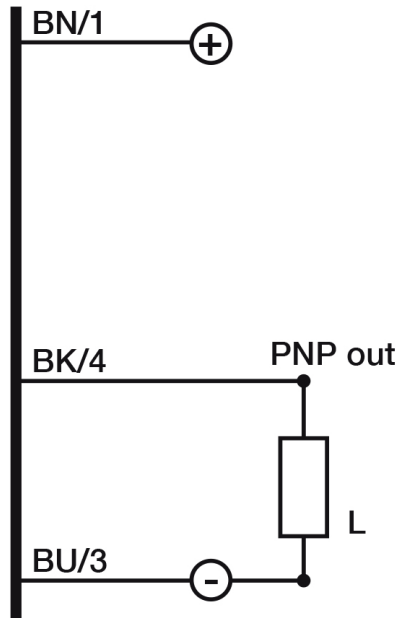
Eletrical diagram
