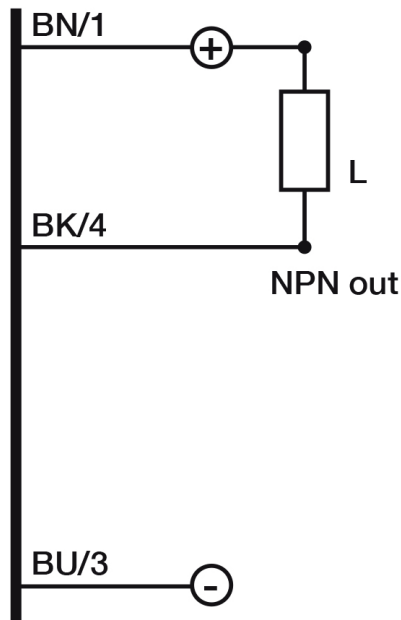
Eletrical diagram
