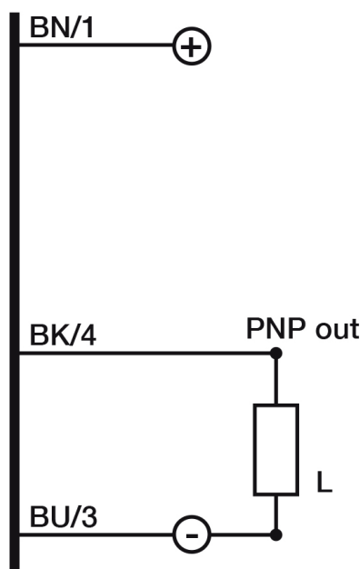
Eletrical diagram
