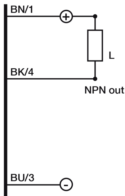
Eletrical diagram
