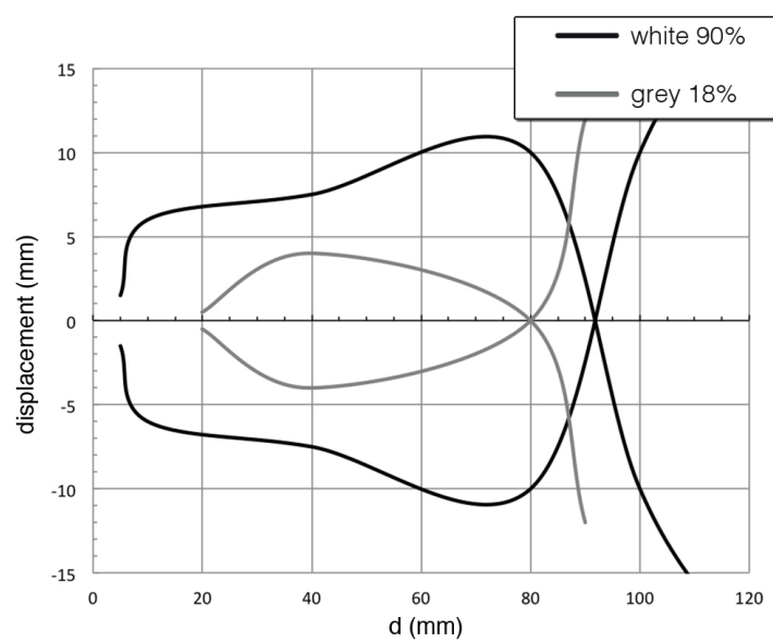
Response curves
