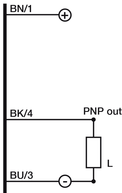
Eletrical diagram
