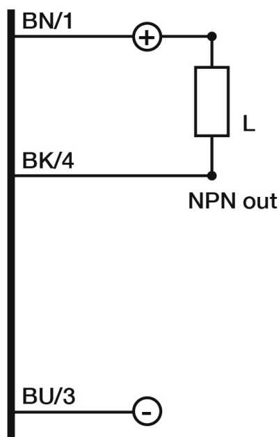
Connector
