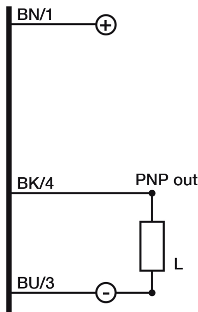
Eletrical diagram
