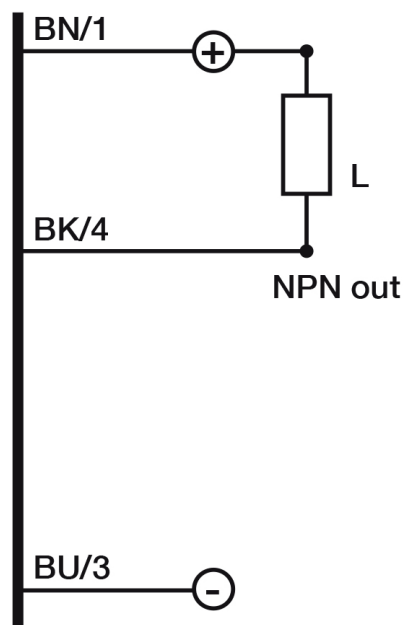
Eletrical diagram
