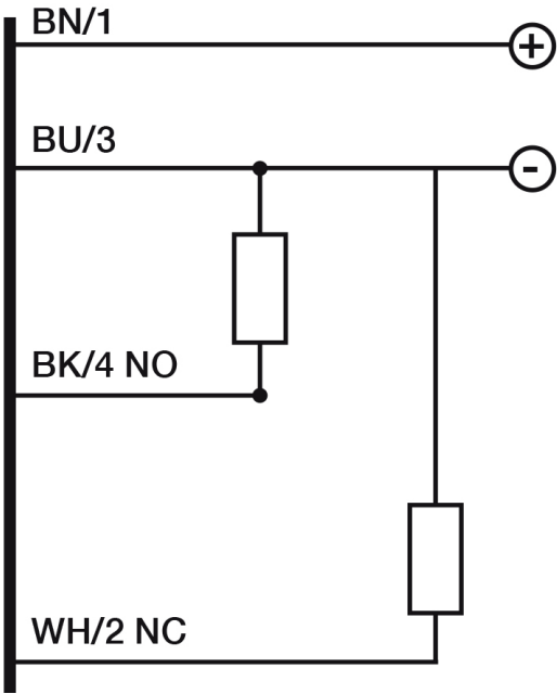
Eletrical diagram
