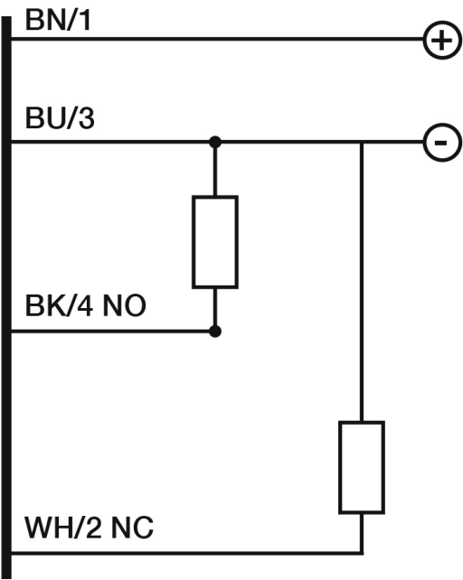
Eletrical diagram
