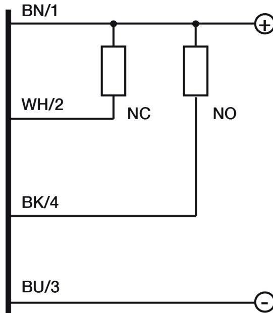
Electrical diagram
