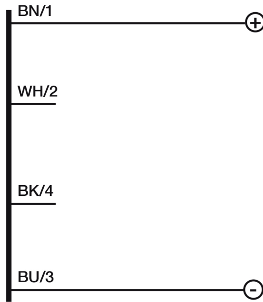
Connector
