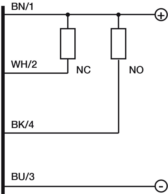
Eletrical diagram
