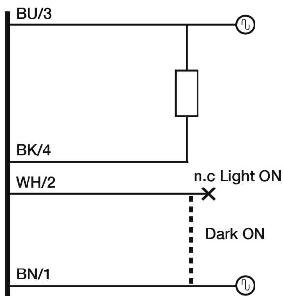
Eletrical diagram
