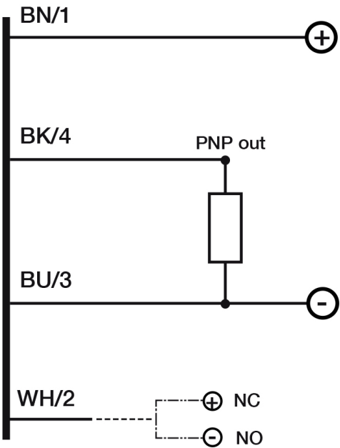
Connector
